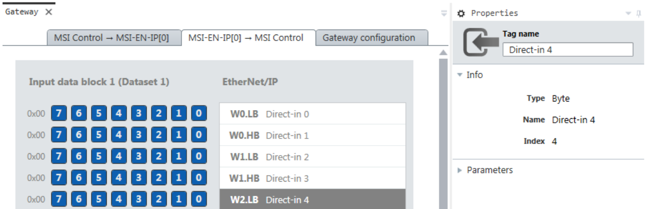
Fig. 8.21: Adding of a new data byte (T→O) for use in the logic editor by configuring the tag name.
