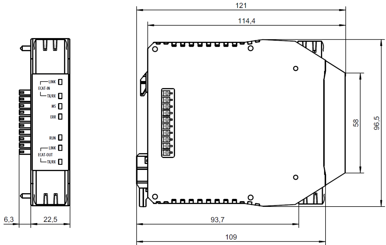
Fig. 12.46: Dimensional drawing EtherCAT gateway (mm)
