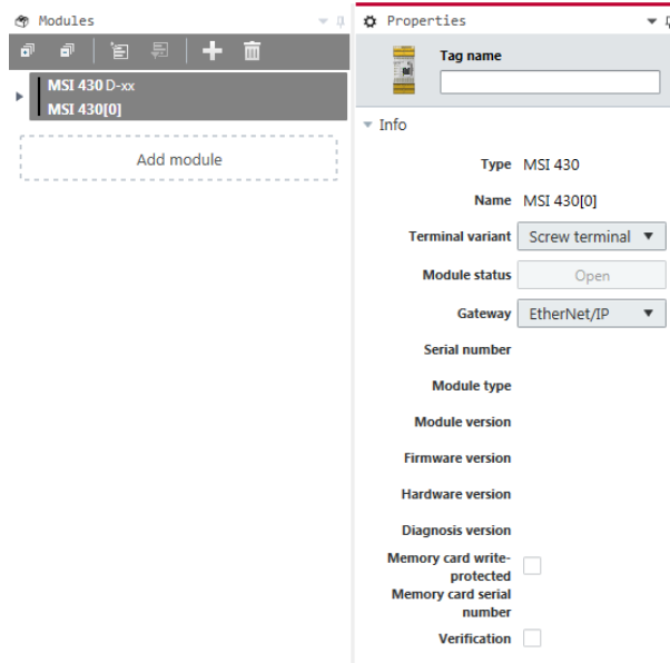
Fig. 8.4: Display of diagnostic version and hardware version in configuration dialog of the controller module
